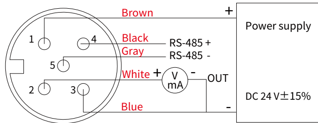
M12 connector
