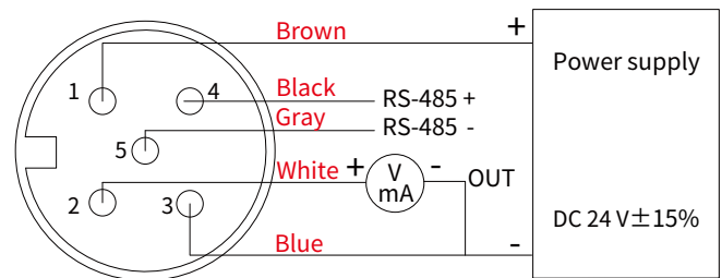
M12 connector
