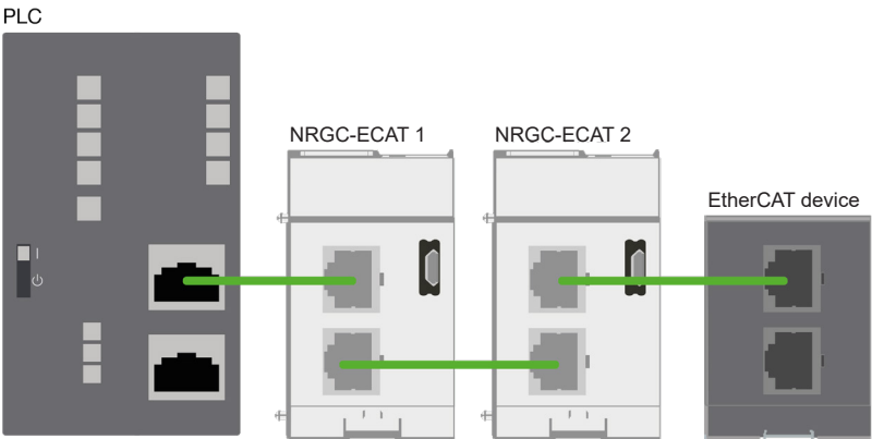
Fig. 3 Example of a line configuration of the NRG-ECAT with other EtherCAT devices and controller
