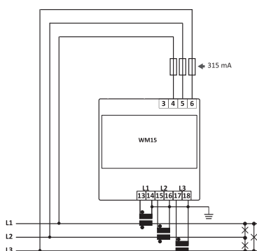
Fig. 8 Three-phase without neutral (3-wire)
