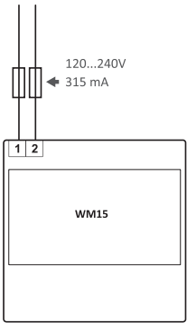
Fig. 13 Auxiliary power supply (H)
