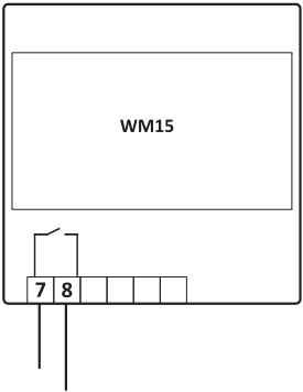
Fig. 14 Digital output
