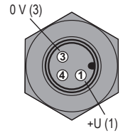
Connection diagram of the ULM level meter (variant –I) and inside view of the connector
