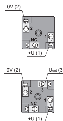
Connection diagram of the ULM level meter (variant -I) and inside view of the connector
