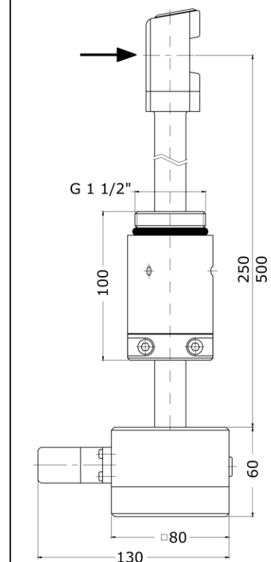
Vortex Flow Sensor VA40
