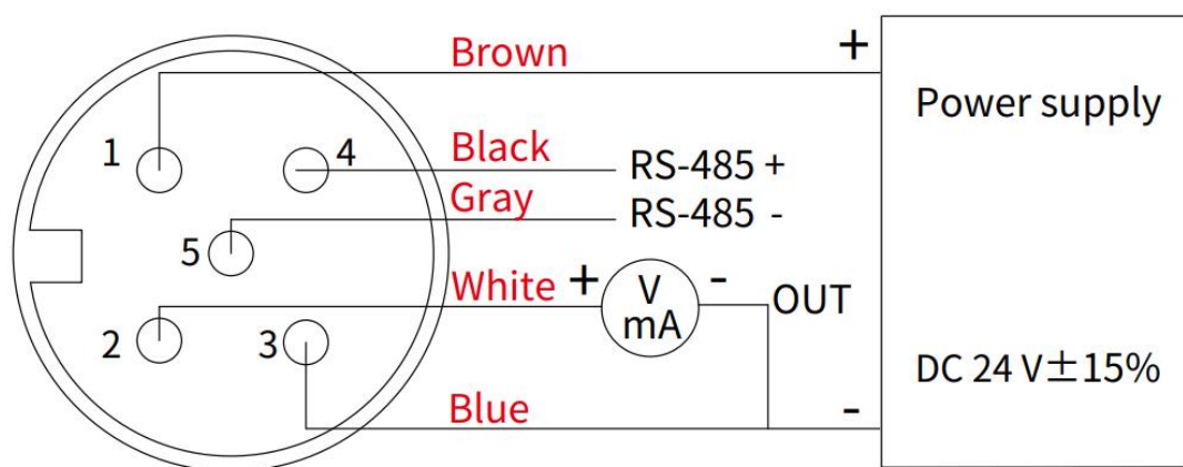
M12 Connector
